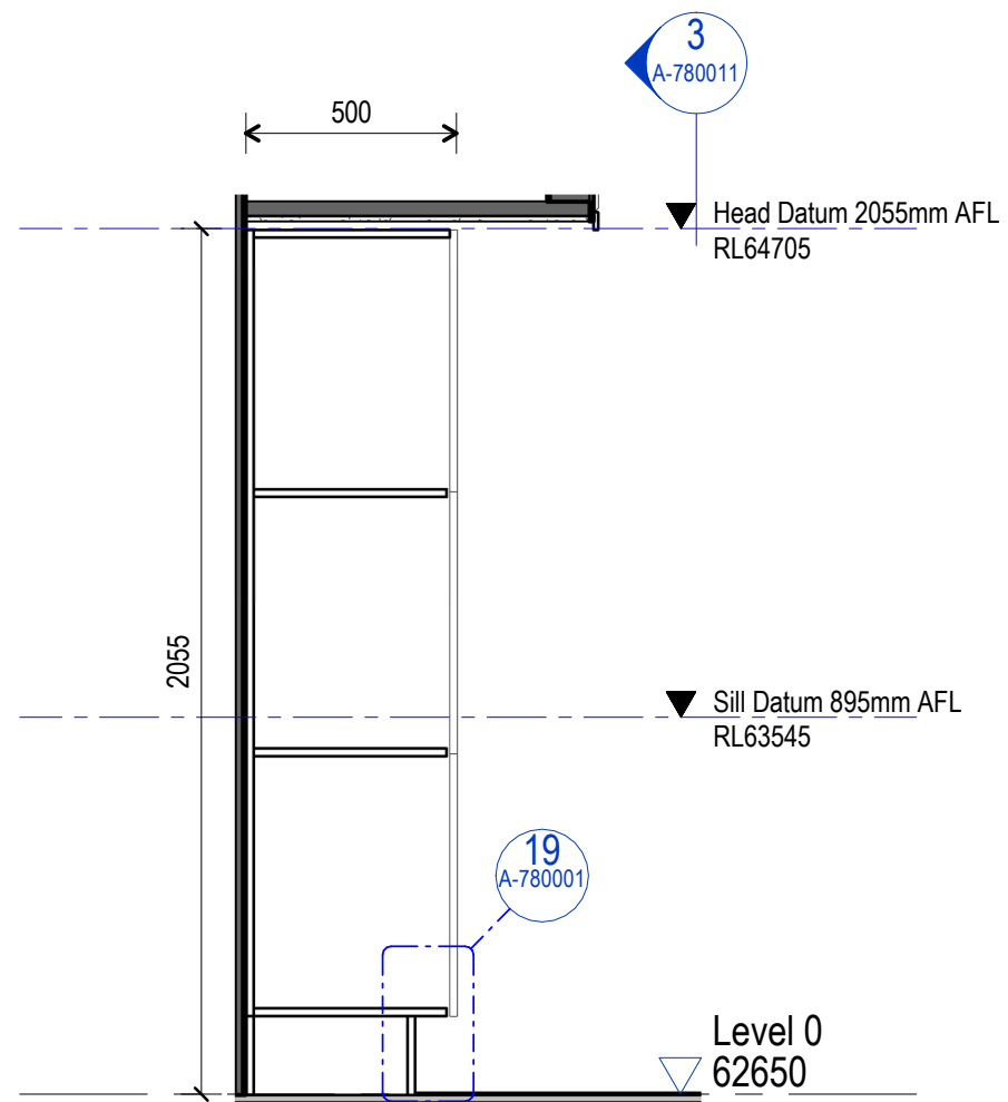
4 JO-LKR-1 Section 1:20
